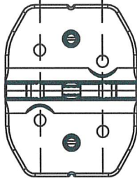
FASTENER PATTERN #1 (2) FASTENERS IN RAFTER
